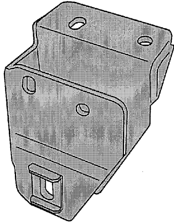
REAR AXLE PIVOT BRACKET F2502-01 / QTY 1
